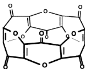
MCS hexamer (C 3 O 2 ) 6
